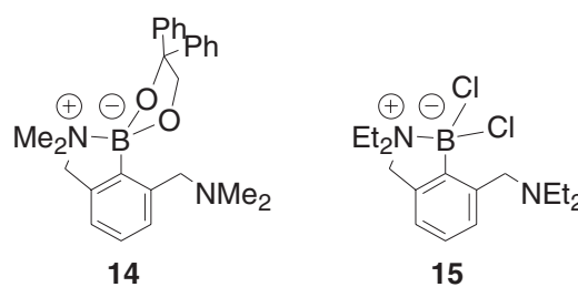
Figure 7. Structures of 14 and 15 .
