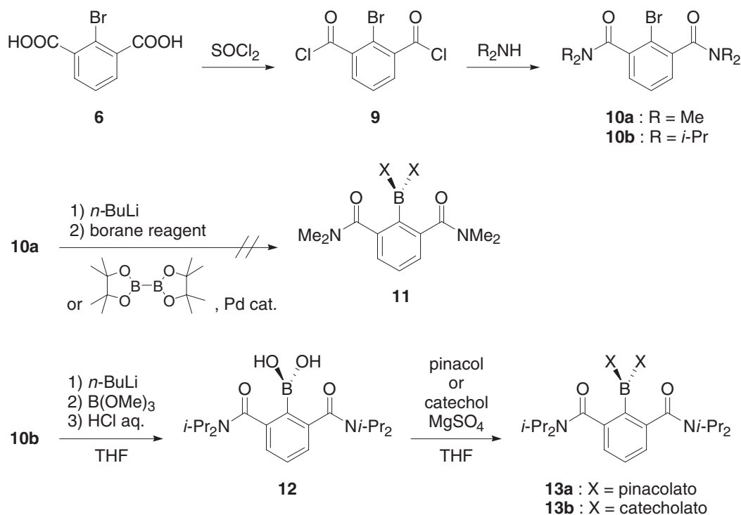
Scheme 2. Preparation of boron compounds using 2,6-bis( N,N -diisopropylaminocarbonyl)phenyl ligand.
