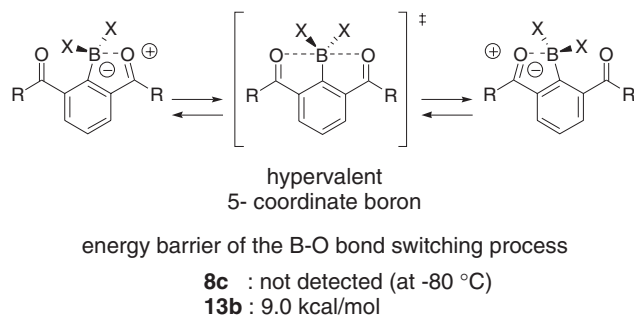
Figure 8. B–N bond switching equilibrium in 8c and 13b .
