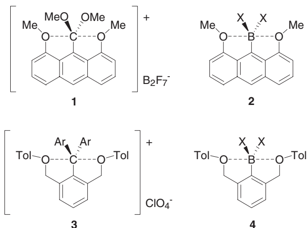
Figure 1. Pentacoordinate carbon and boron compounds.
