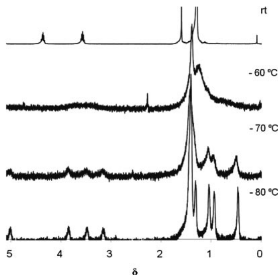
Figure 9. Variable-temperature ^1\text{H} NMR ( \text{CD}_2\text{Cl}_2 ) spectra of 13b .
