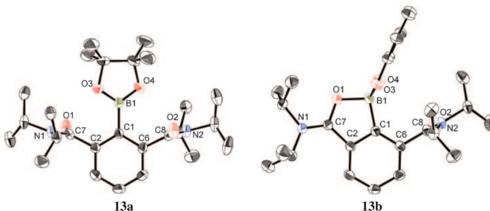
Figure 5. ORTEP drawings of 13a and 13b (50% thermal ellipsoid; all hydrogen atoms and water for 13b are omitted for clarity).
