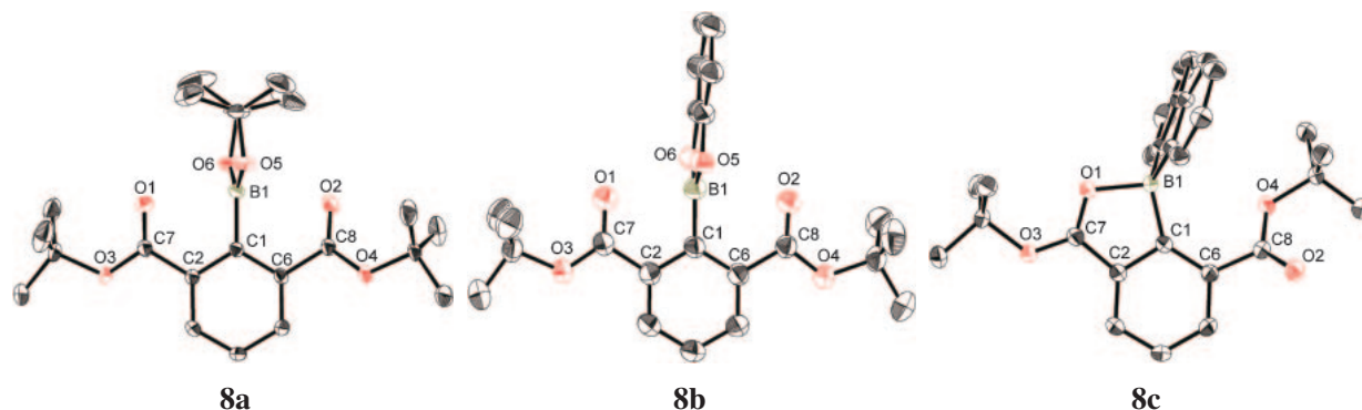
Figure 4. ORTEP drawings of 8a , 8b , and 8c (50% thermal ellipsoid; all hydrogen atoms and 2-hydroxy-4,4,5,5-tetramethyl-1,3,2-dioxaborolane for 8a are omitted for clarity).
