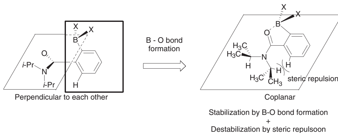
Figure 6. Steric repulsion between diisopropylamide group and benzene ring.
