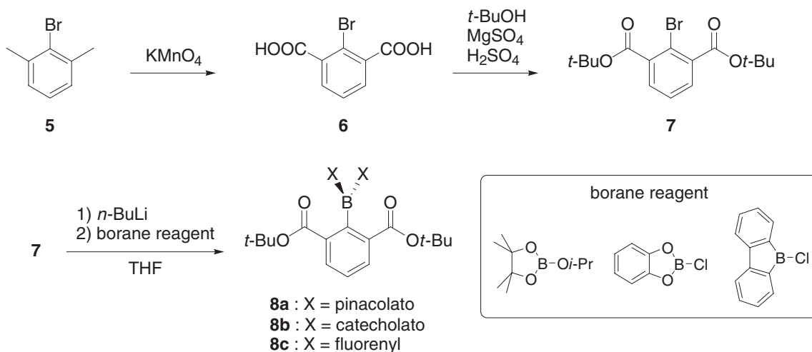
Scheme 1. Preparation of boron compounds using 2,6-bis( t -butoxycarbonyl)phenyl ligand.
