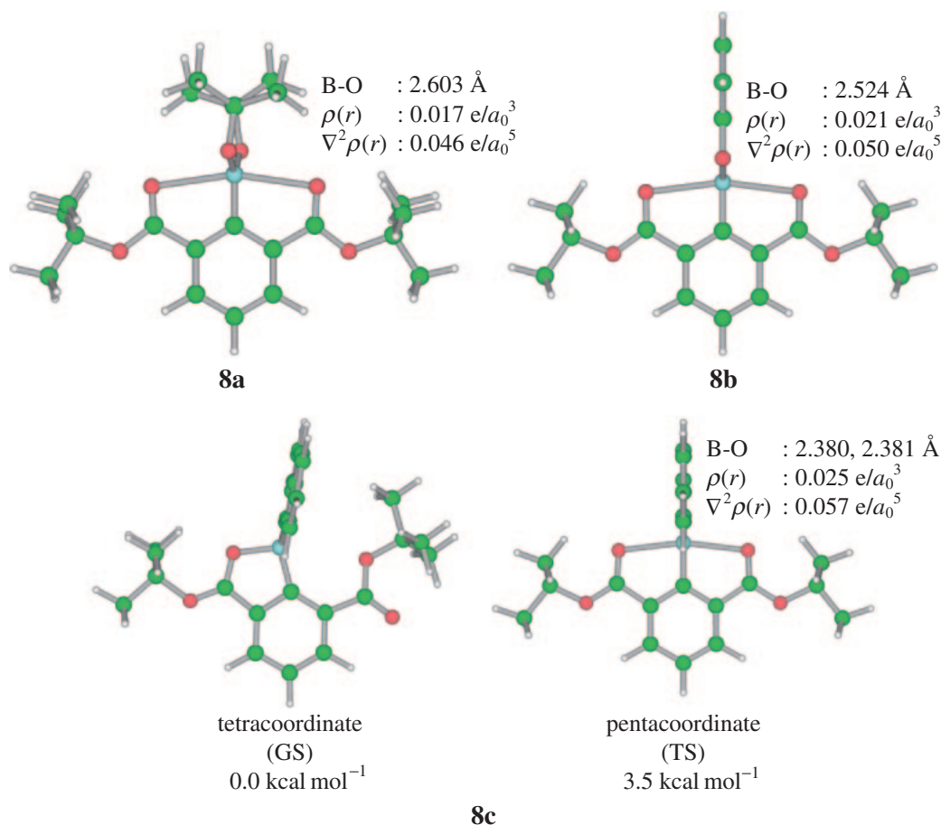
Figure 10. Optimized structures and the AIM data of 8a–8c at the B3PW91/6-31G(d) level.
